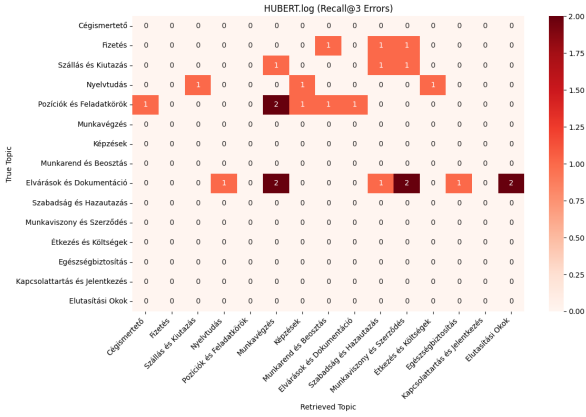
Fig. 10. Confusion matrix for the HUBERT model
