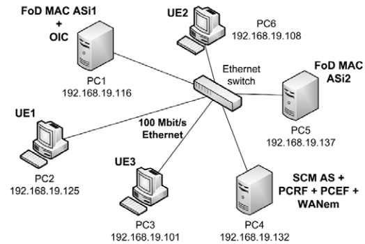
Fig. 5. Topology of the experimental testbed
