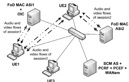
Fig. 6. Flow map after establishing sessions
