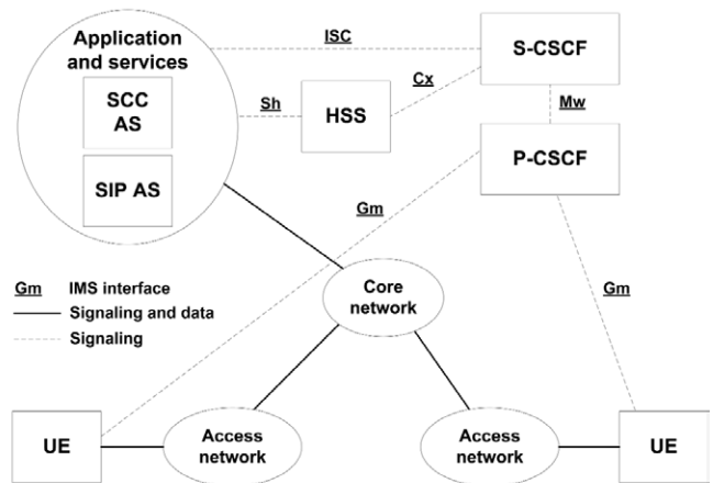
Fig. 1. A simplified view of the 3GPP IMS architecture
