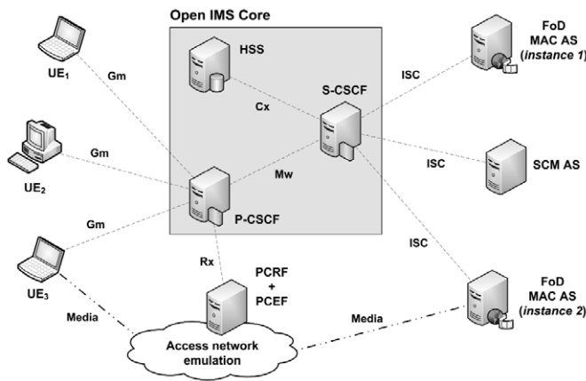
Fig. 2. Architecture of the IMS-based laboratory prototype
