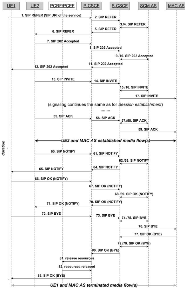
Fig. 4. SIP signaling for Session reconfiguration upon a change of terminal
