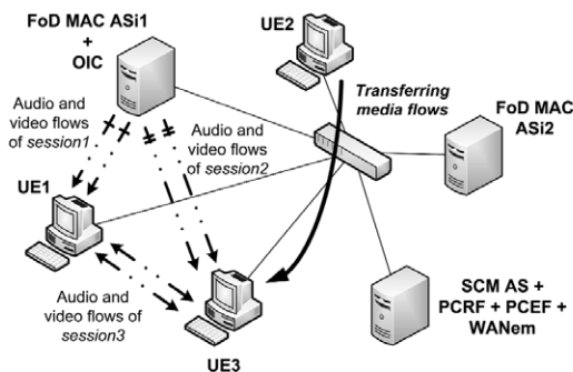
Fig. 7. Flow map after transferring media flows
