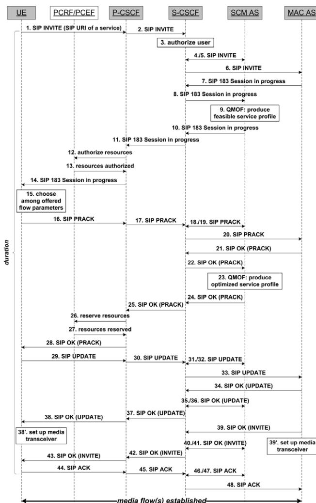
Fig. 3. SIP signaling for Session establishment
